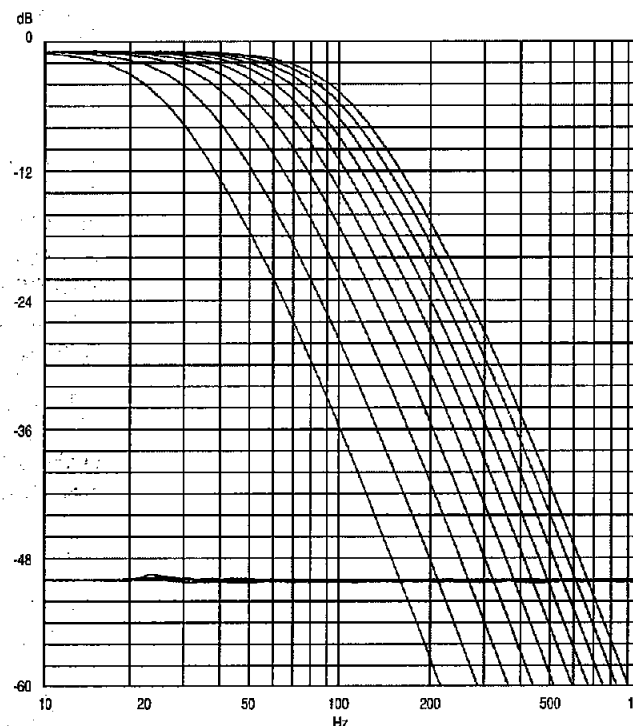
Lowpass Filter
