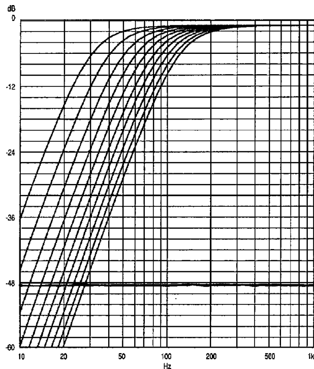
Highpass Filter
